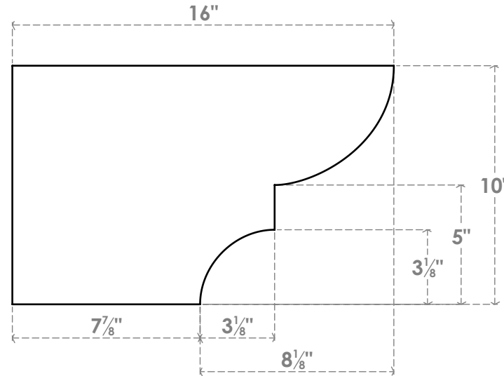
SIDE PROFILE
